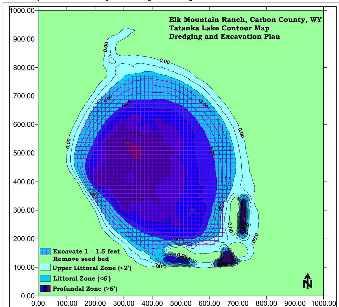
Diagram 6: Dredging and Excavation Plan for Tatanka Lake
