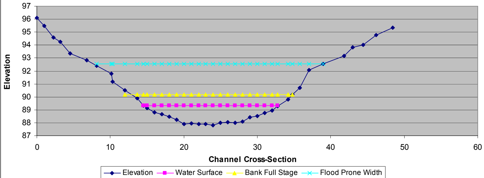
Fountain Creek - Manitou Springs Reach 2 - Fields Park - Cross Section #1a
