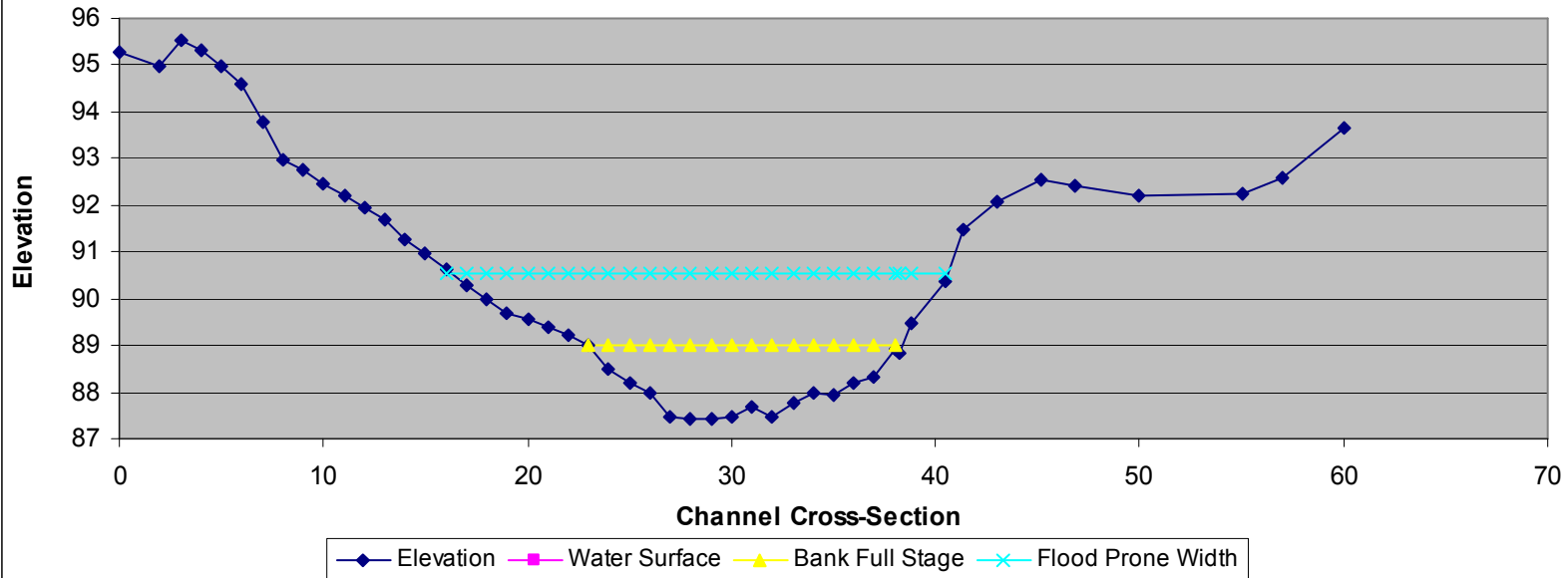
Fountain Creek - Manitou Springs Reach 2 - Fields Park - Cross Section #1
