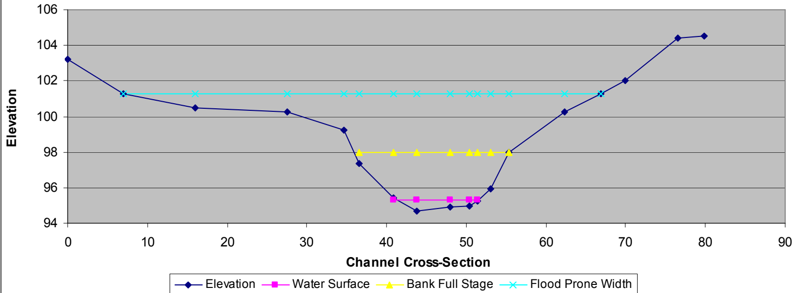
Fountain Creek - Manitou Springs Reach 2 - Fields Park - Cross Section #3
