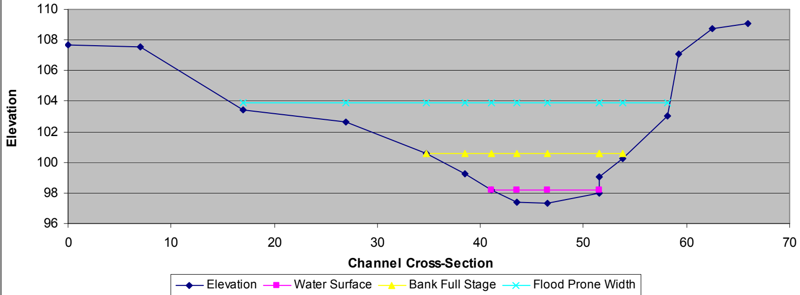
Fountain Creek - Manitou Springs Reach 2 - Fields Park - Cross Section #4
