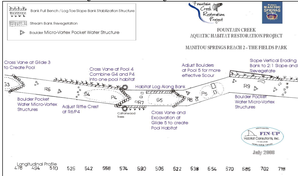
Plan view of Habitat enhancements and bank stabilization from Glide 3 through Riffle 9 of Reach 2 of Fountain Creek within The Fields Park.
