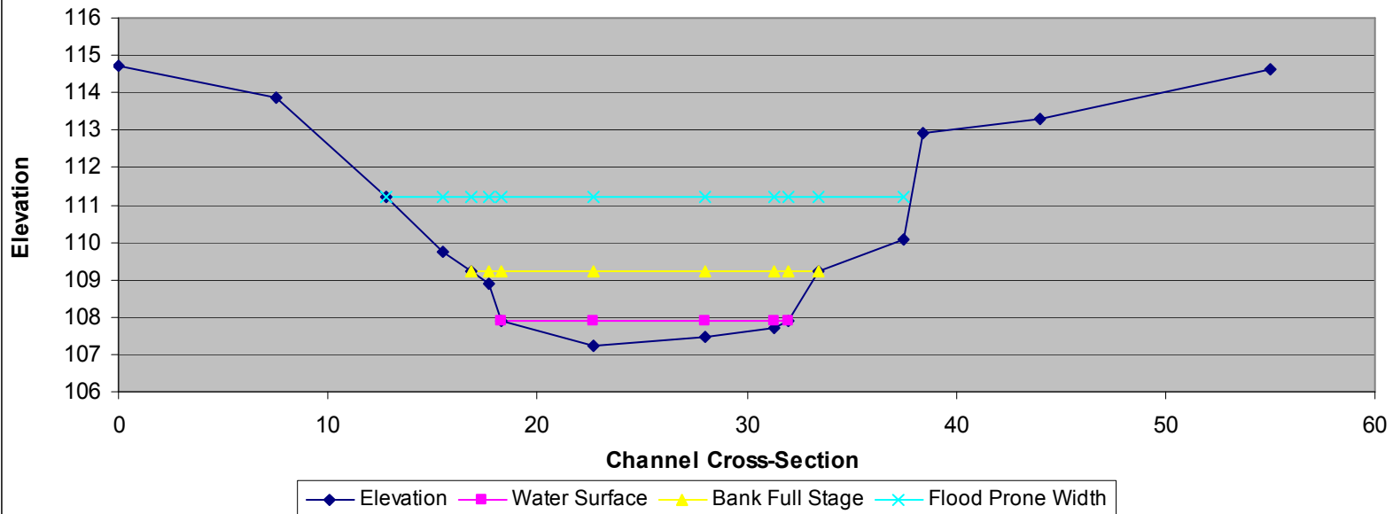
Fountain Creek - Manitou Springs Reach 2 - Fields Park - Cross Section #5
