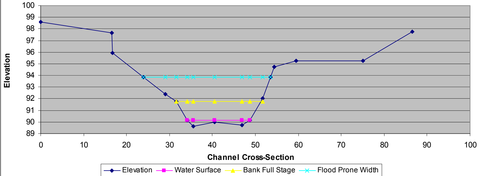
Fountain Creek - Manitou Springs Reach 2 - Fields Park - Cross Section #2
