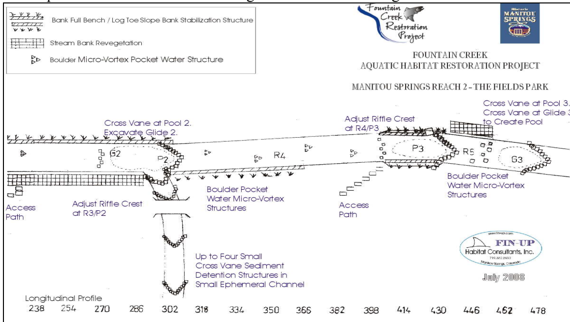
Plan view of Habitat enhancements and bank stabilization from Glide 2 through Glide 3 of Reach 2 of Fountain Creek within The Fields Park.
